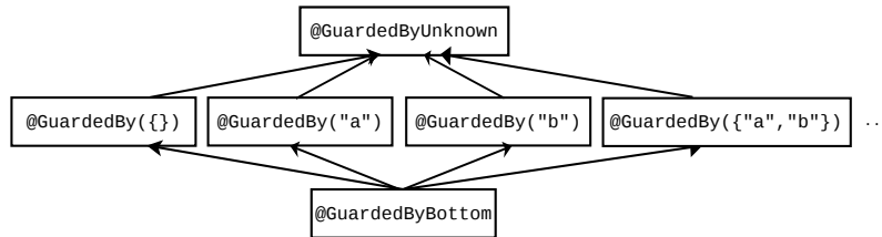
Figure 11.1: The subtyping relationship of the Lock Checker's qualifiers. @GuardedBy({}) is the default type qualifier for unannotated types (except all CLIMB-to-top locations other than upper bounds and exception parameters — see Section 31.5.3).
