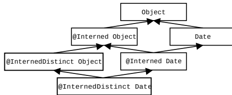
Figure 5.1: Type hierarchy for the Interning type system.
