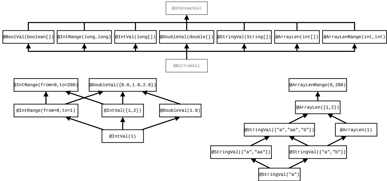
Figure 17.1: At the top, the type qualifier hierarchy of the Constant Value Checker annotations. Qualifiers in gray are used internally by the type system but should never be written by a programmer. At the bottom are examples of additional subtyping relationships that depend on the annotations' arguments.
