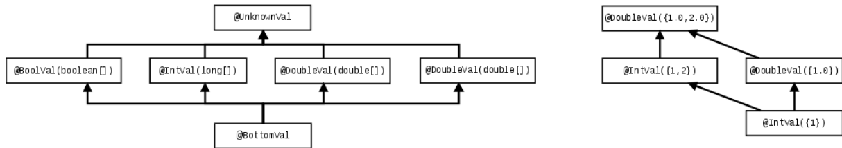
Figure 17.1: The type qualifier hierarchy of the Constant Value Checker annotations. Qualifiers in gray are used internally by the type system but should never be written by a programmer. On the right are examples of additional subtyping relationships that depend on the annotations' arguments.
