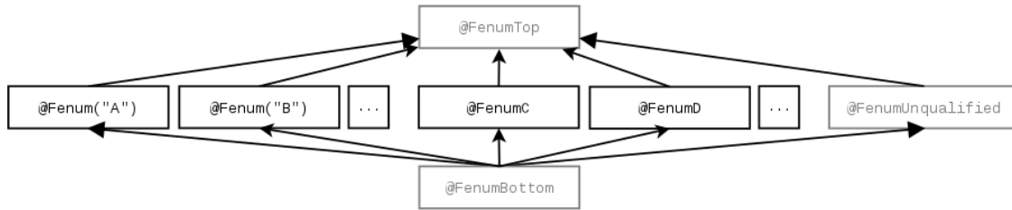
Figure 7.1: Partial type hierarchy for the Fenum type system. There are two forms of fake enumeration annotations — above, illustrated by @Fenum("A") and @FenumC . See Section 7.1 for descriptions of how to introduce both types of fenums. The type qualifiers in gray ( @FenumTop , @FenumUnqualified , and @FenumBottom ) should never be written in source code; they are used internally by the type system. @FenumUnqualified is the default qualifier for unannotated types, except for upper bounds which default to @FenumTop .
