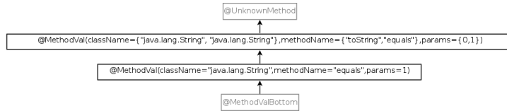
Figure 20.2: Partial type hierarchy for the MethodVal type system. The type qualifiers in gray (@UnknownMethod and @MethodValBottom) should never be written in source code; they are used internally by the type system.
