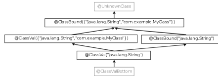
Figure 20.1: Partial type hierarchy for the ClassVal type system. The type qualifiers in gray (@UnknownClass and @ClassValBottom) should never be written in source code; they are used internally by the type system.
